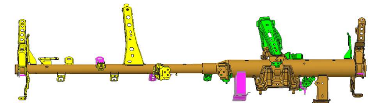
INSTRUMENT PANEL REINFORMENT TUBE
