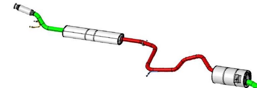
SELTOS COLD END SILENCER
